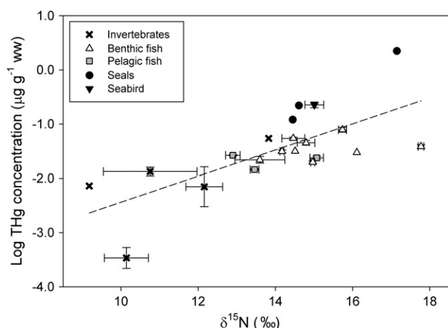
Fig. 4. Relationship between \delta^{15}\text{N} ratios (‰) and log-transformed THg concentrations ( \mu\text{g g}^{-1}\text{ ww} ) in a marine food web of Hudson Bay (linear regression model: \log \text{THg} = 4.84 + 0.240 * \delta^{15}\text{N} , r^2 = 0.49 , p < 0.001 , n = 21 ). Invertebrates (sea angel ( Clione limacina ), jellyfish (mixed species), squid ( Gonatus sp.), amphipods (gammarid and hyperiid), euphausiids (Euphausiacea), pelagic fish (Arctic cod ( Boreogadus saida ), capelin ( Mallotus villosus ), sand lance ( Ammodytes spp.), and benthic fish (sculpins ( Gymnancistrus tricuspid , Triglops spp.), banded gunnels ( Pholis fasciata ), Arctic and daubed shannies ( Stichaeus punctatus and Leptoclinus maculatus , respectively), eelpout ( Gymnelis viridis ), Atlantic poacher ( Leptogobius decagonus ), fourline snake blennies ( Eumesogrammus praecisus ), snailfish ( Liparis sp.)) were sampled from 2007 to 2009. Seabirds (thick-billed murre) were sampled in 2007. Ringed seals were sampled in 2006, bearded seals ( Erignathus barbatus ) in 2005, and harbor seals ( Phoca vitulina ) from 1999 to 2006. Fish data are from Braune et al. (2014a). Invertebrate and seabird data are from Braune (Environment Canada, unpublished data). Seal data are from Young et al. (2010).
